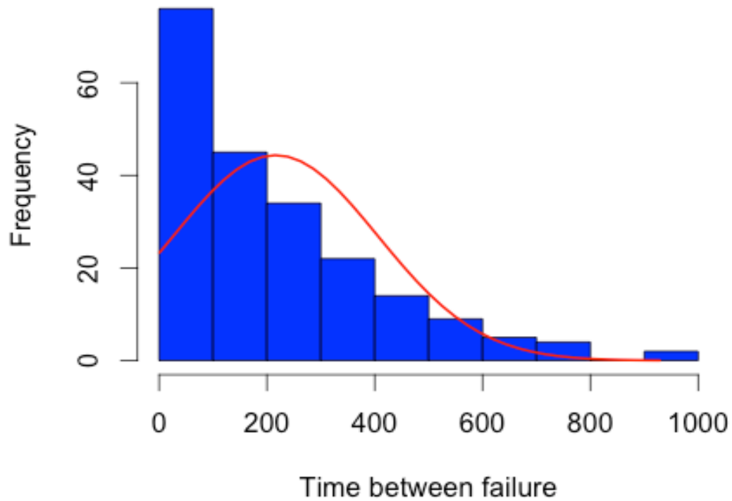
Figure 2: Product Returns Frequency Graph of Time Between Failures (in days)
